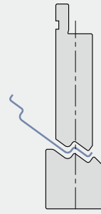
16. Crash-forming joggle (Z) tool with short flange
