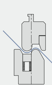
31. Adjustable joggle (Z) tool with spring loaded ejector
