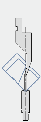
1. Punch/top-tool and die for special profile
