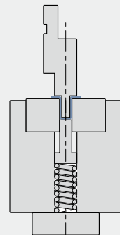
20. Top-hat-bending tool with bending strips and spring loaded ejector
