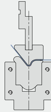
28. Crash-forming tool in avothene insert with form punch (mark free)
