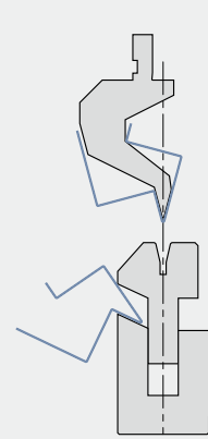
4. Pre-bending and flattening tool with spring loaded die
